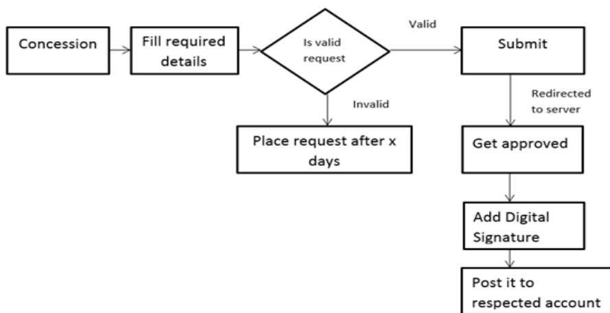
figure.3: Placing request for concession
